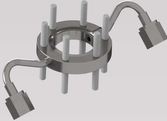
XT ConFlat to VCR Adapter with 2 adapter arms (P/N: ADDSCFVCR2V2)
